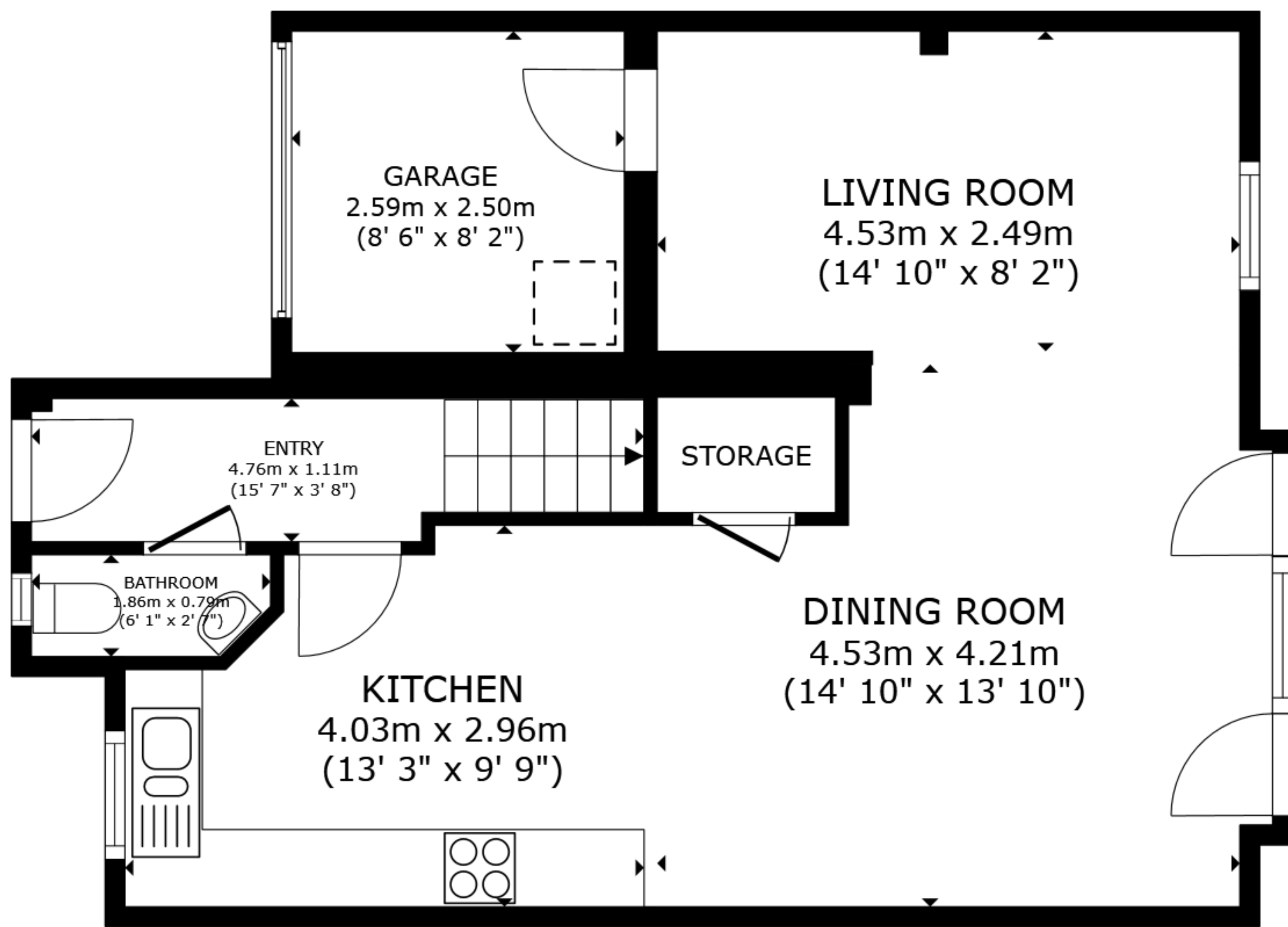
FLOOR 1
