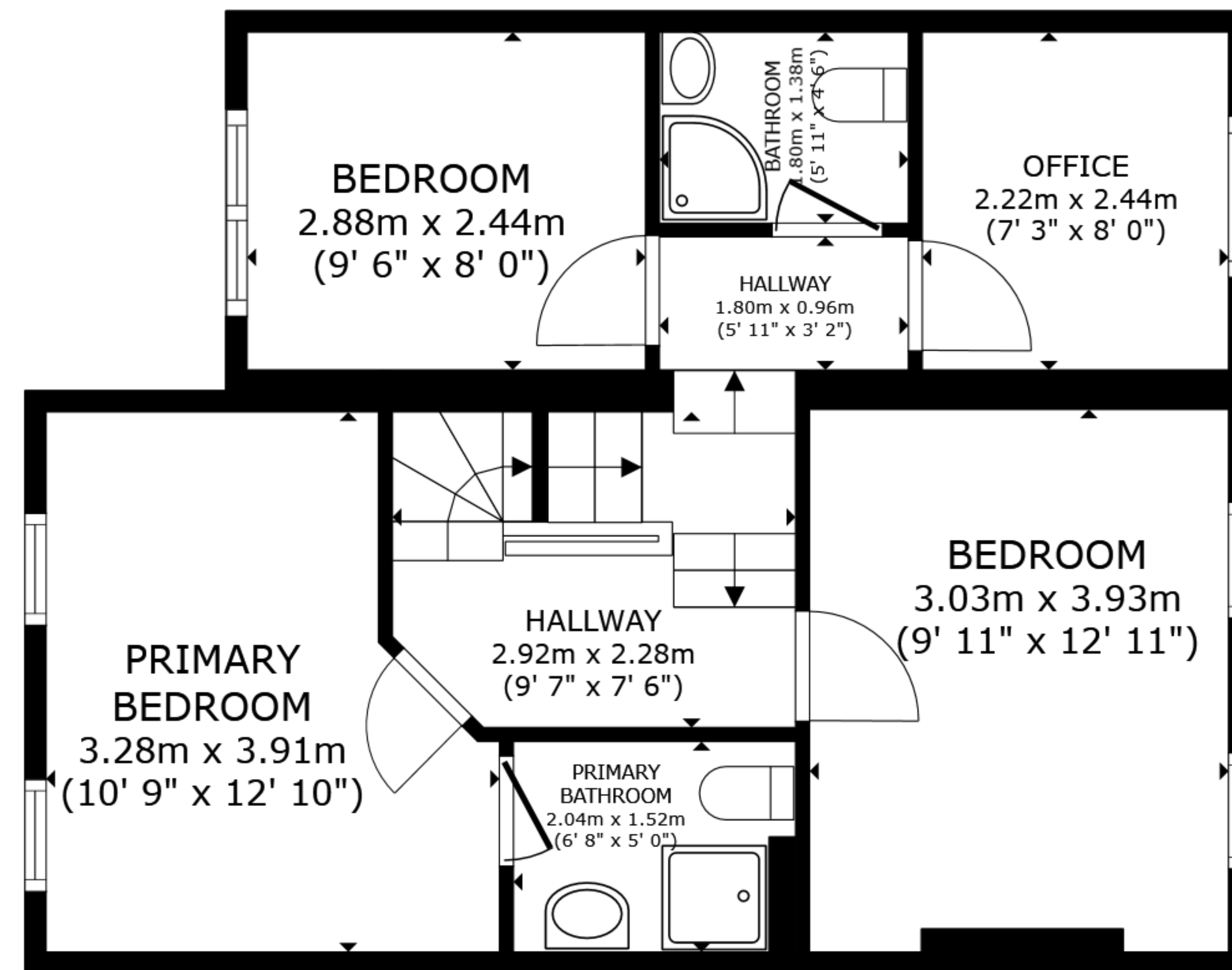
FLOOR 2
